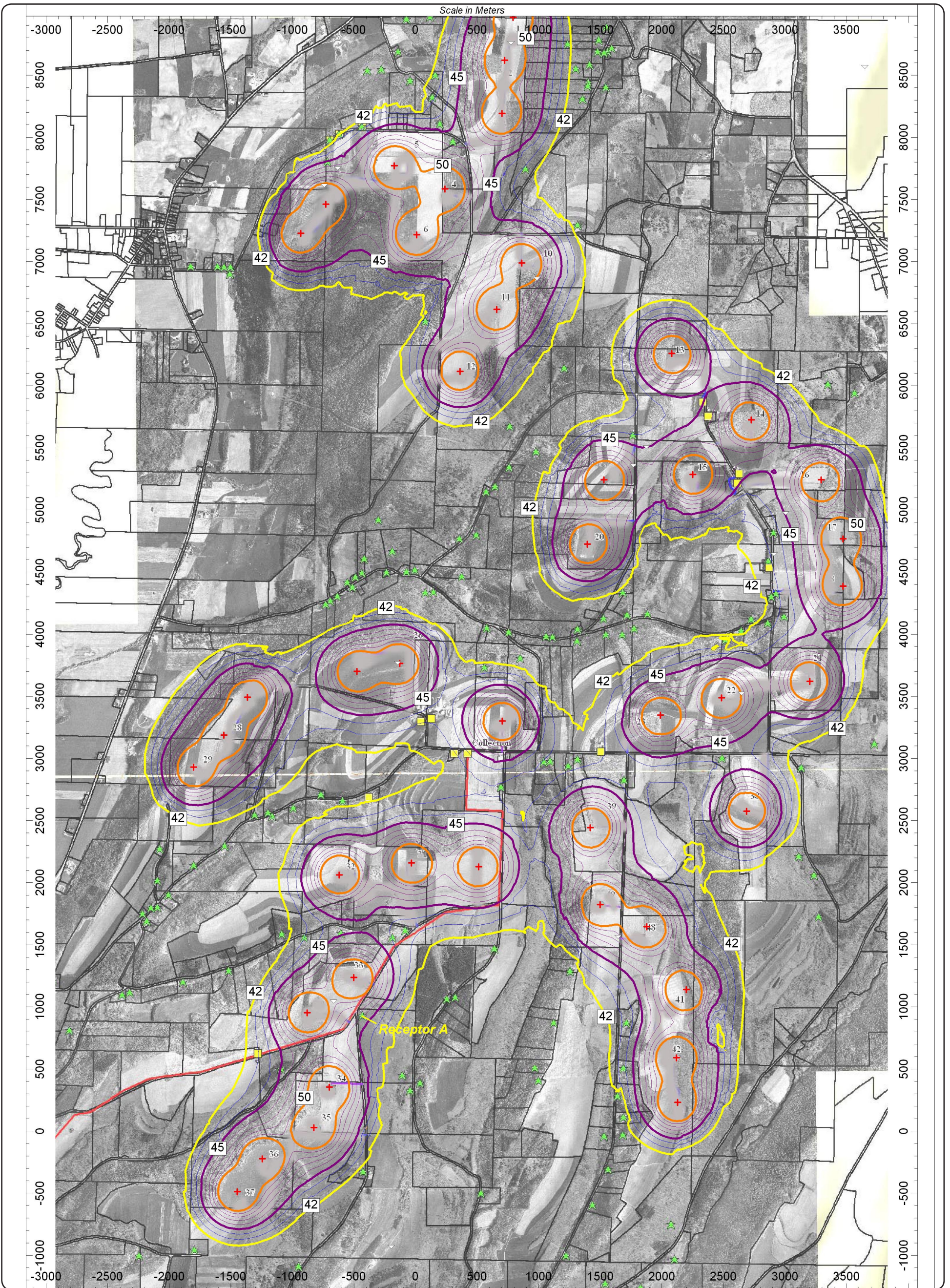
Figure 18: Predicted Sound Contours (dBA) Assuming an Omnidirectional 8 m/s Wind Sheet 1 of 2 Cohocton Wind Power Project
