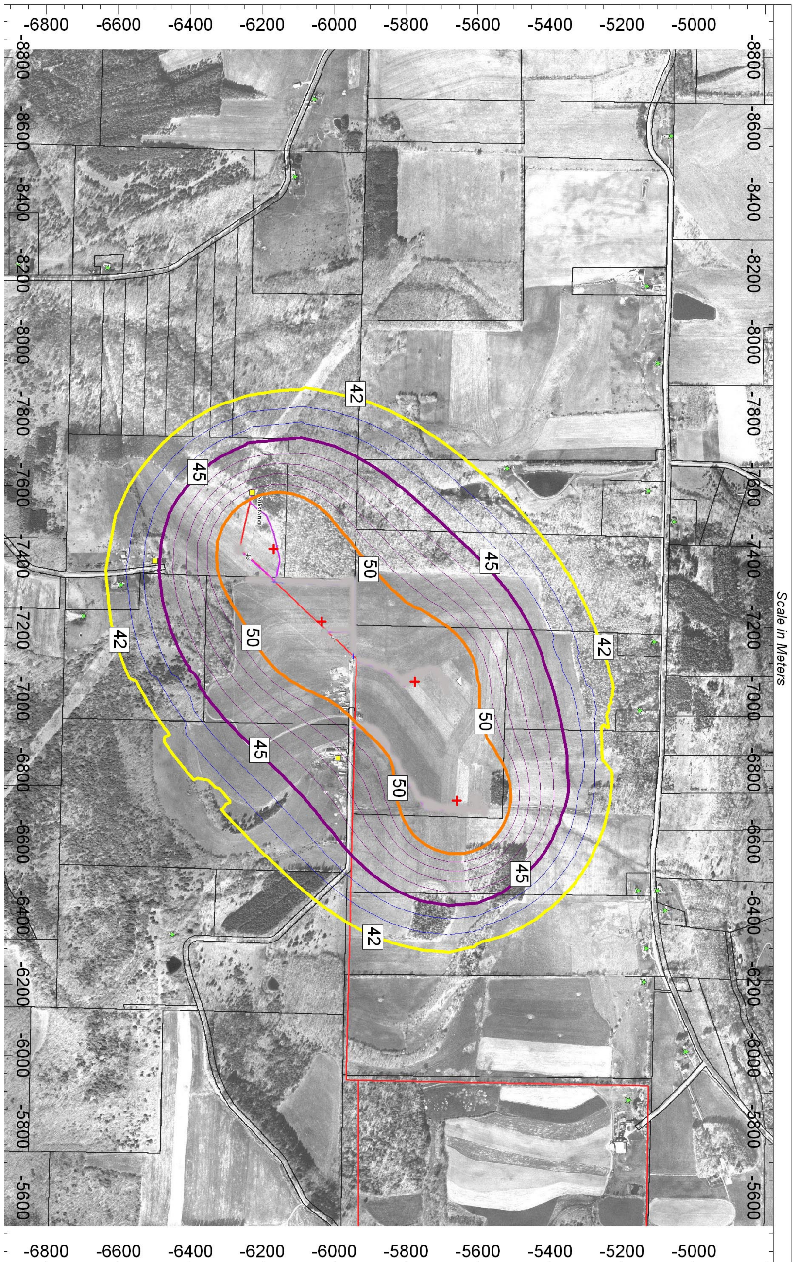
Figure 18: Predicted Sound Contours (dBA) Assuming an Omnidirectional 8 m/s Wind Sheet 2 of 2 Cohocton Wind Power Project
