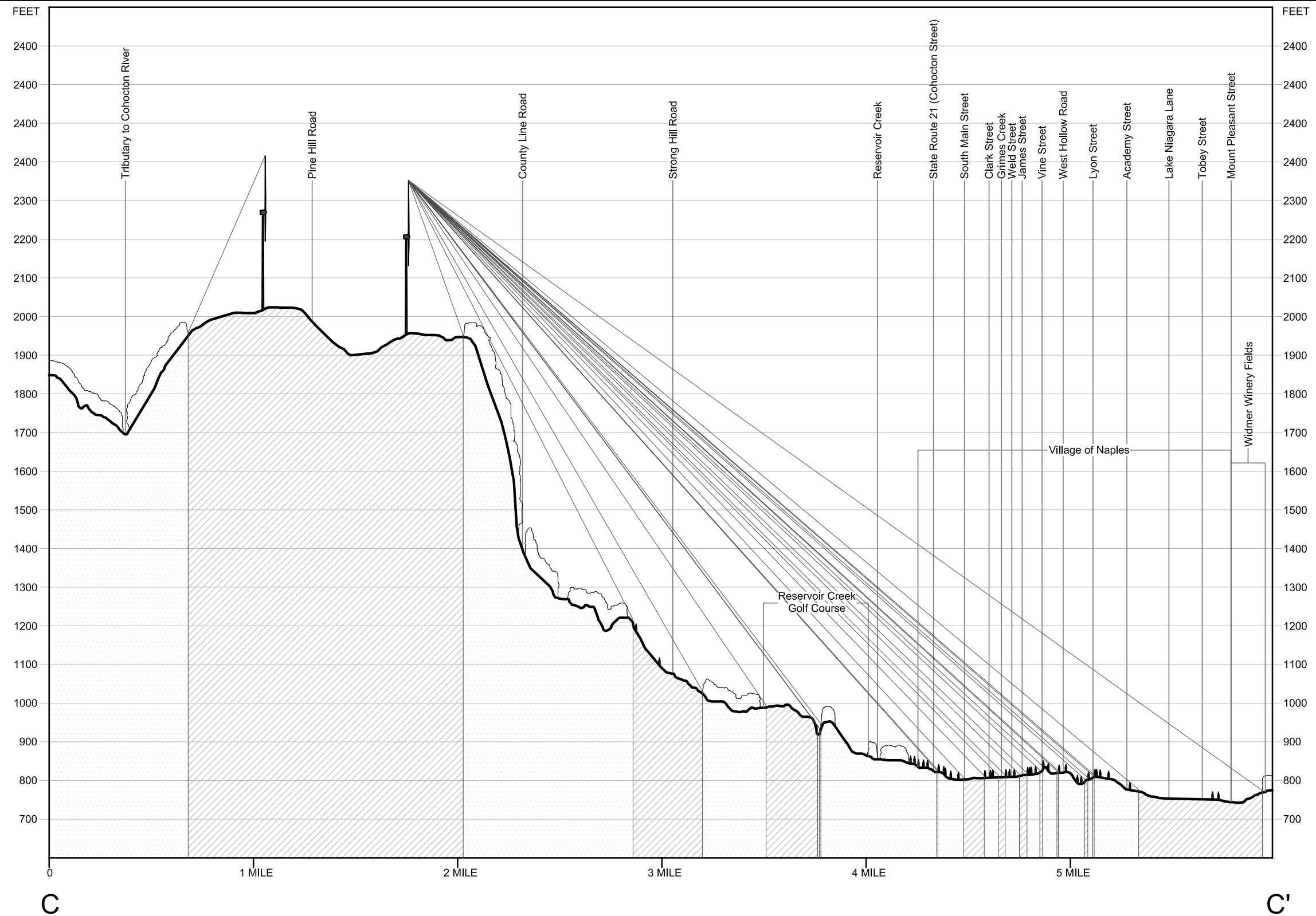
Figure 7: Line of Sight Cross Sections Sheet 4 of 5 - Section C - C'
