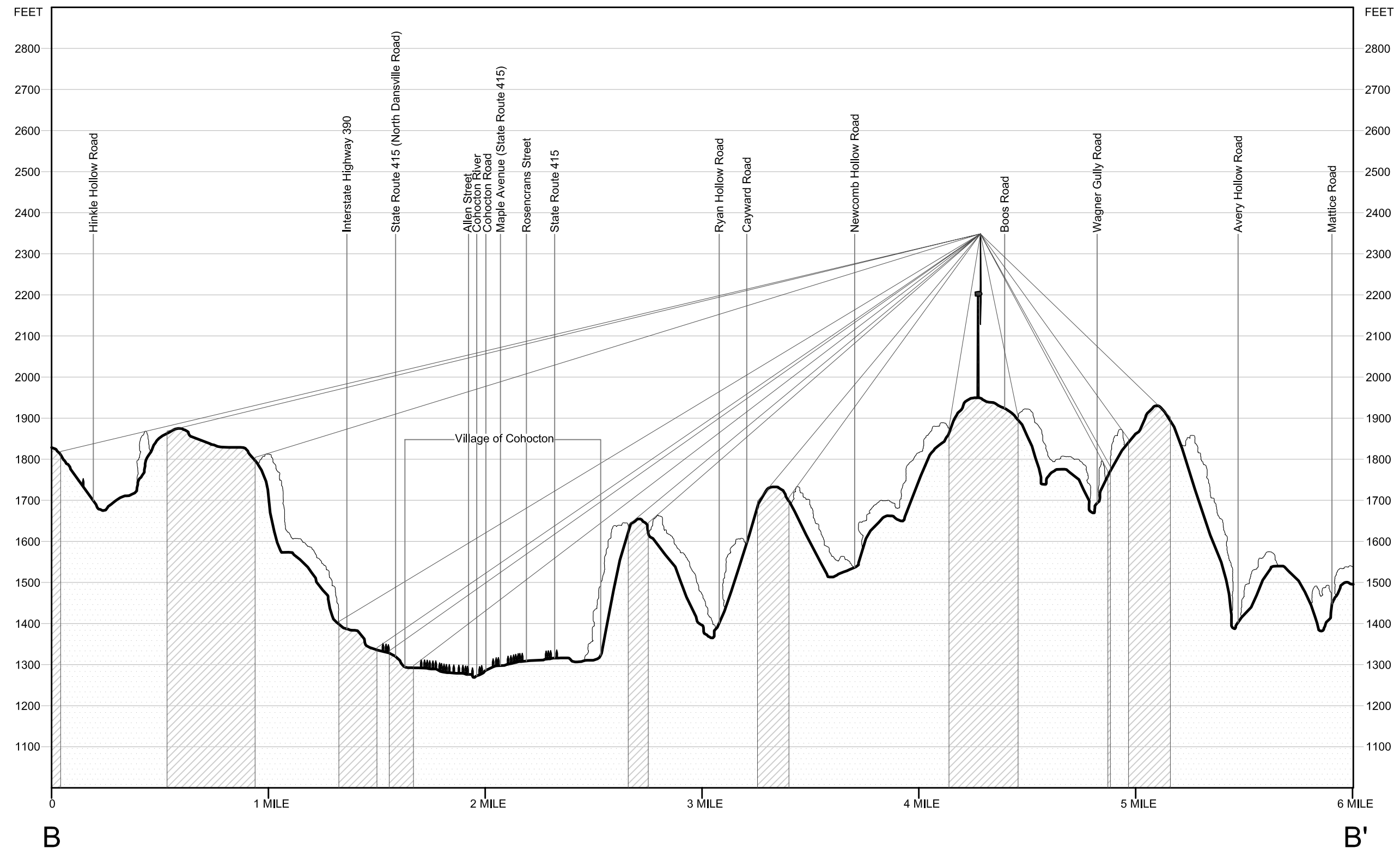
Figure 7: Line of Sight Cross Sections Sheet 3 of 5 - Section B - B'
