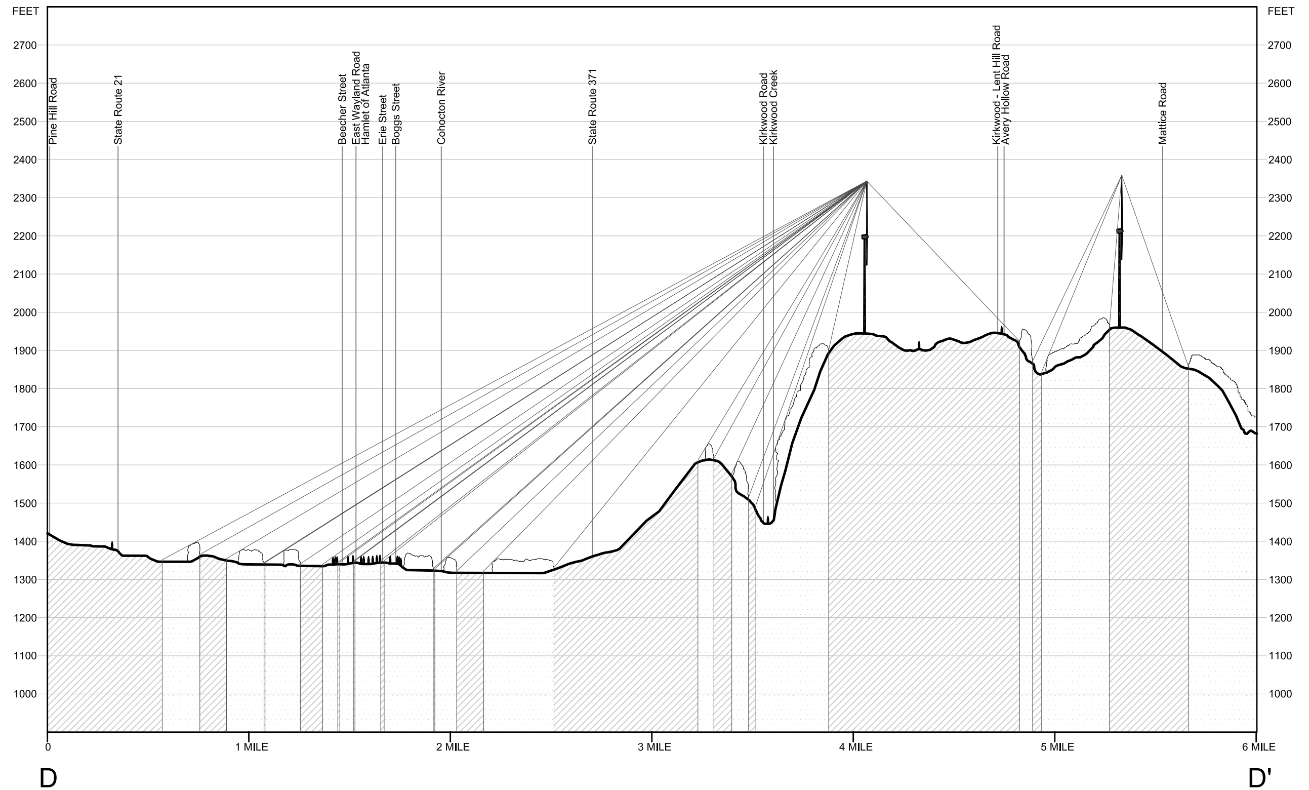
Figure 7: Line of Sight Cross Sections Sheet 5 of 5 - Section D - D'
