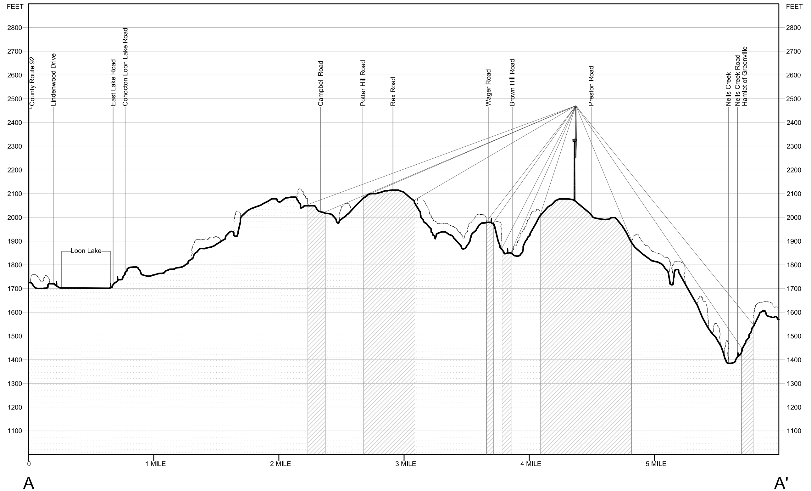
Figure 7: Line of Sight Cross Sections Sheet 2 of 5 - Section A - A'
