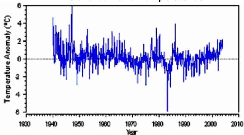
IPCC Greenland Temperatures
